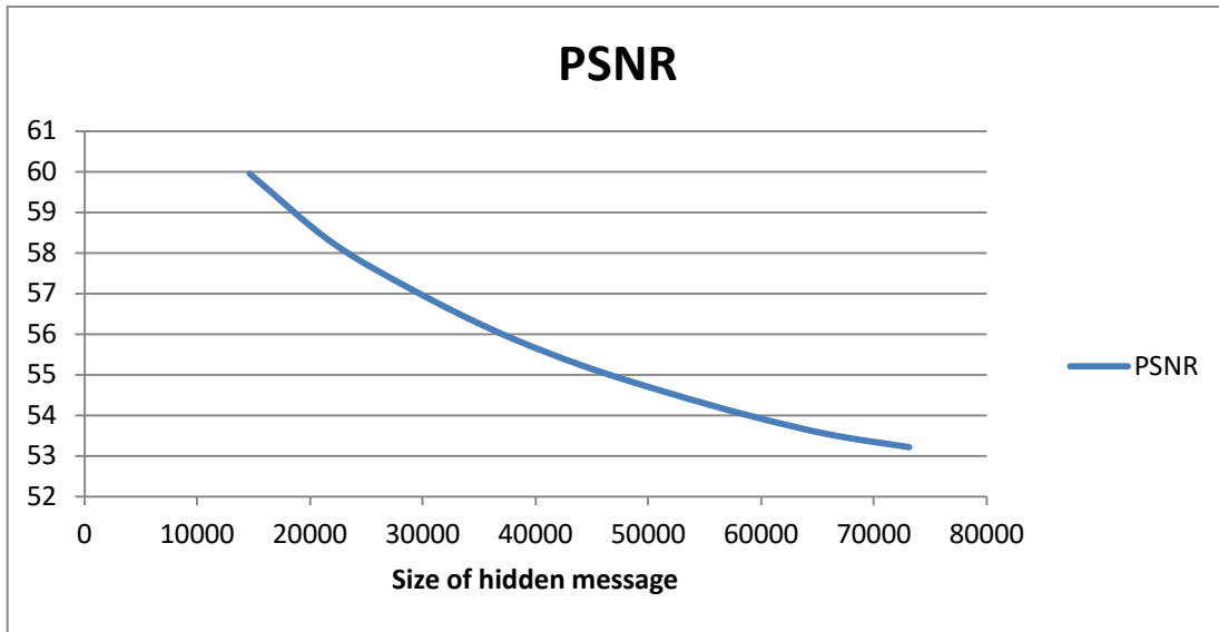
Figures (5.9): The PSNR values for Peppers image
